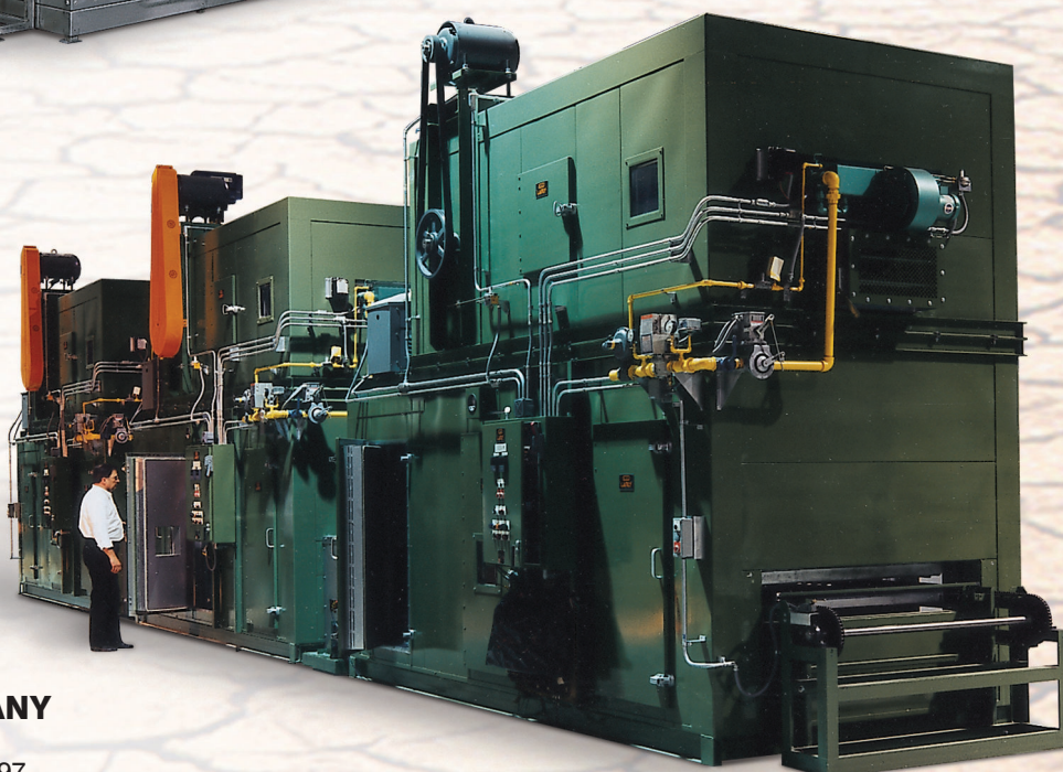
3 ZONE PARTS CURING OVEN
