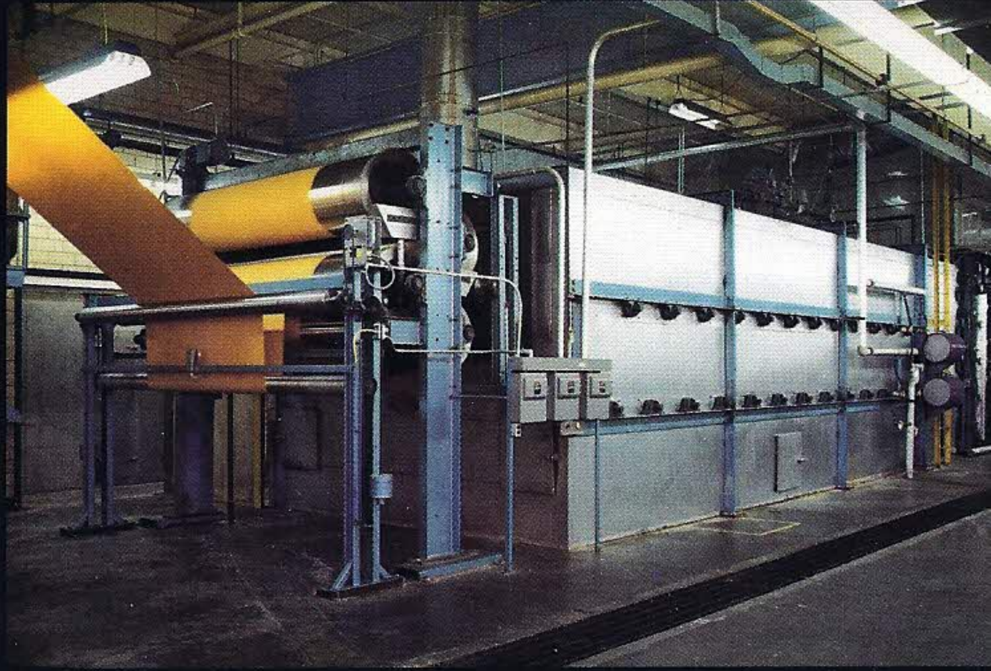
Semi- Contact Thermosol Oven
